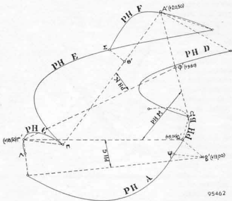
Fig. 4. GENERAL plan
