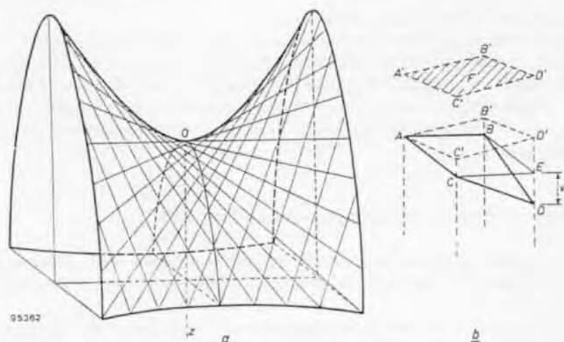
FIG. 6 a) The double-system of generatrices of a hyperbolic paraboloid b) Part of the surface delimited by the intersection of four generatrices: AB, CD, AC, BD
