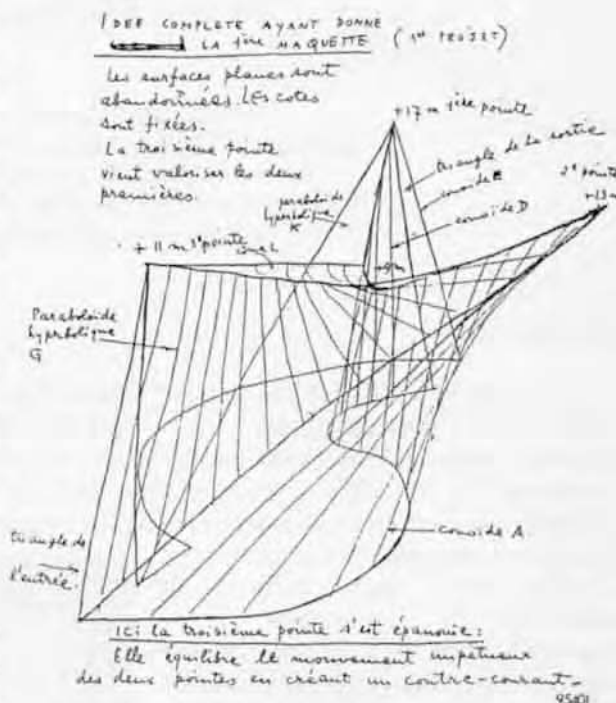
Fig. 2. First project. Sketch by I. Xenakis
